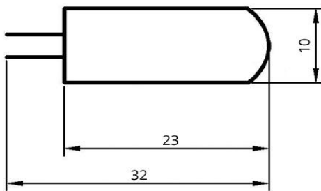
G4 1.5 Watt 12V
